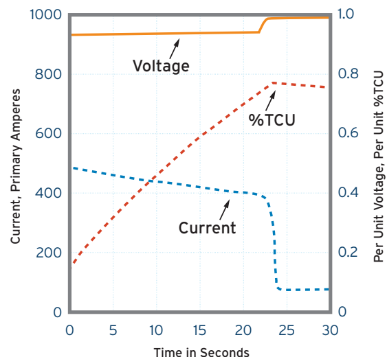
Motor start report data exported to a plotting program.
