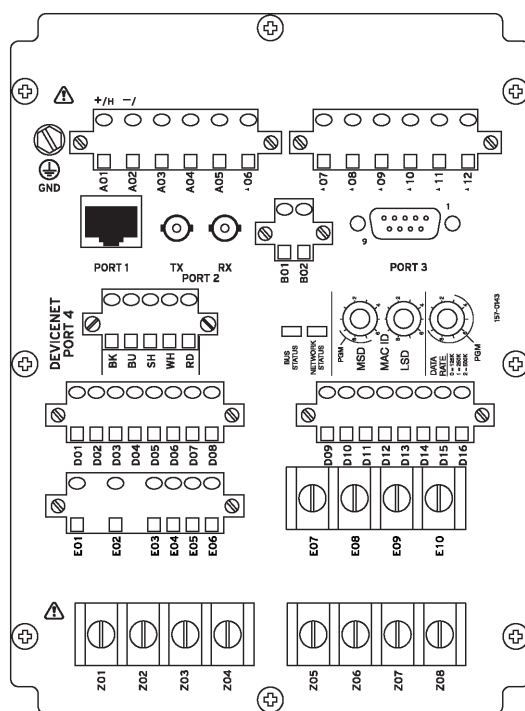
Figure 14 PTC, DeviceNet, 4 DI/4 DO, and Voltage Differential Option
