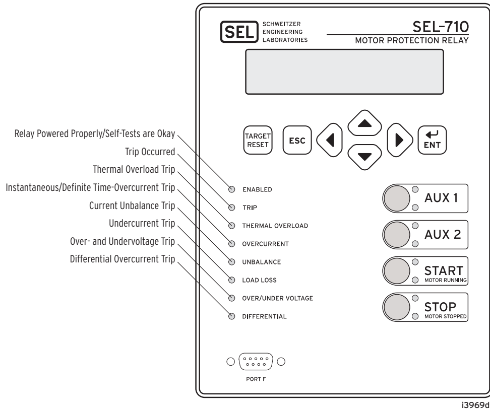
Figure 11 Front Panel
