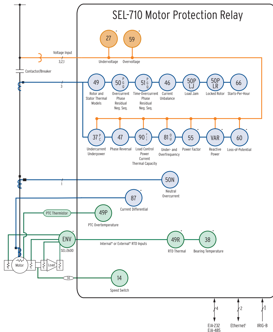
Figure 1 Functional Diagram
