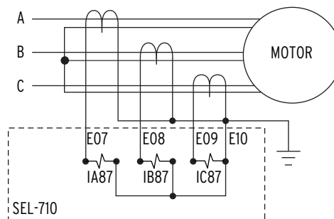
Figure 16 AC Connections With Core-Balance Differential CTs
