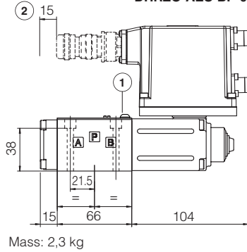
DHRZO-AES-BC-010 DHRZO-AES-BP-010
