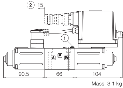
DHRZO-AEB-NP-012
