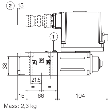
DHRZO-AEB-NP-010
