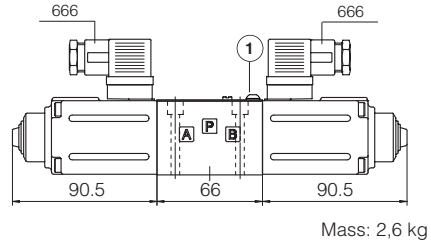
DHRZO-A-012
