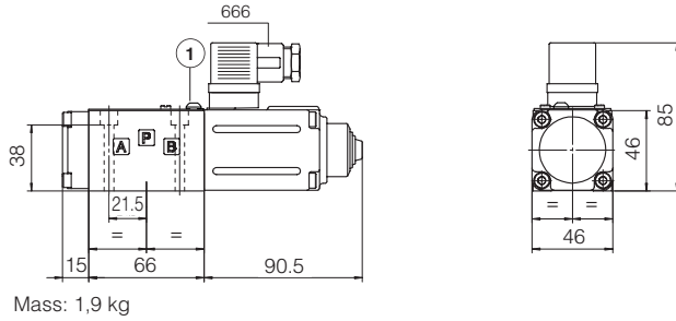
DHRZO-A-010
