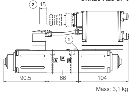
DHRZO-AES-BC-012 DHRZO-AES-BP-012
